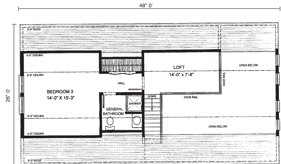
Suggested Second Floor Layout
