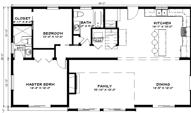
1ST FLOOR
