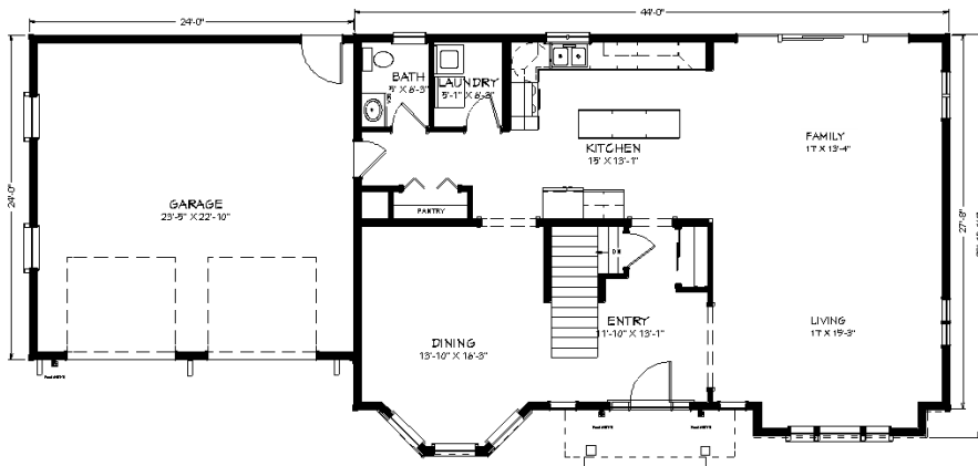
1ST FLOOR
