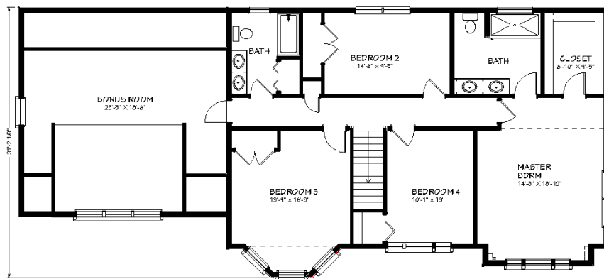
2ND FLOOR
